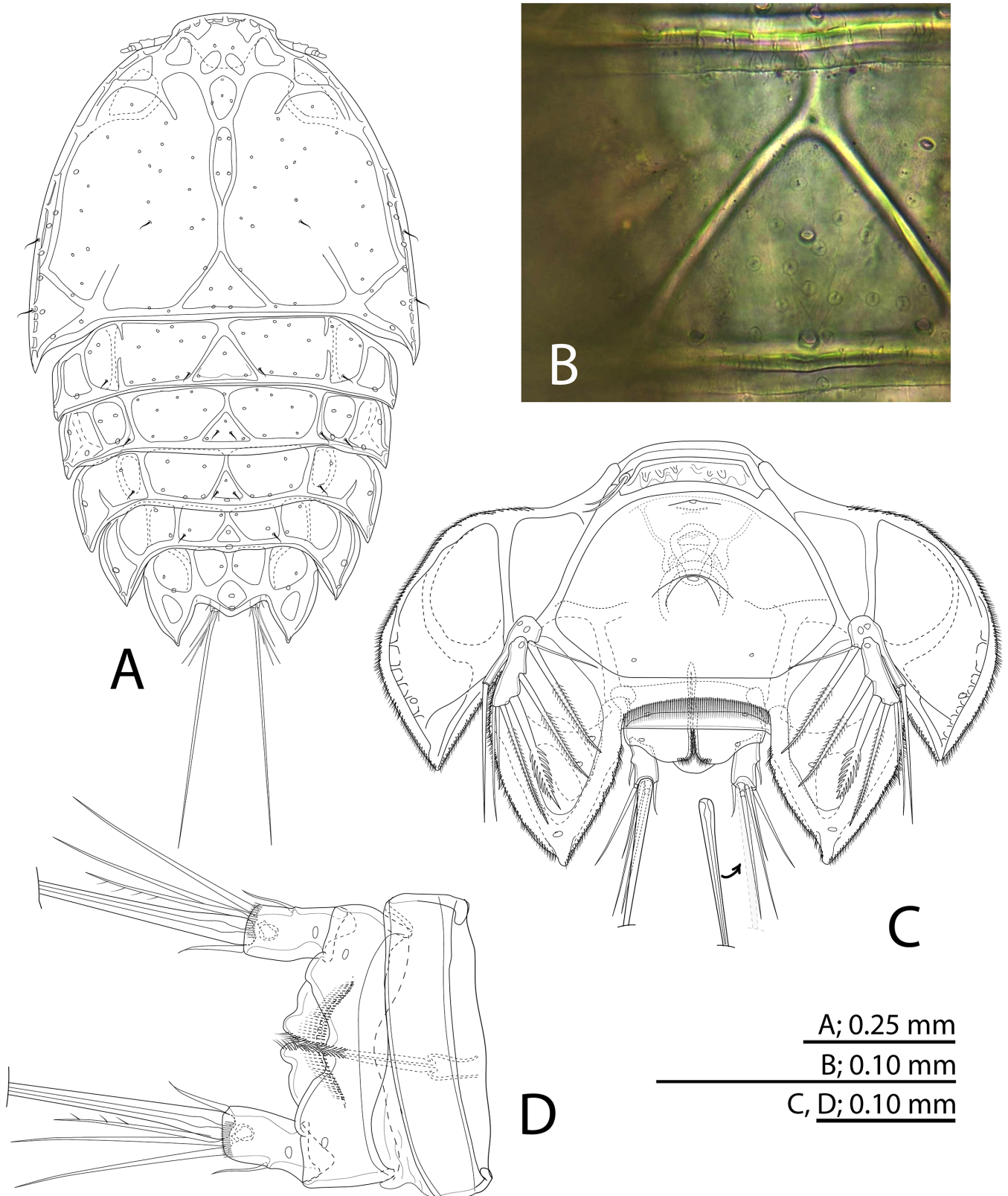
Fig. 3. Peltidium penyu , new species, female holotype (UKMMZ-1638). A, habitus, dorsal view; B, photomicrograph of body integument at the area of second thoracic somite; C, urosome, ventral view; D, second free abdominal somite and anal somite with caudal rami after they were exposed by slightly compressing the urosome, ventral view.
