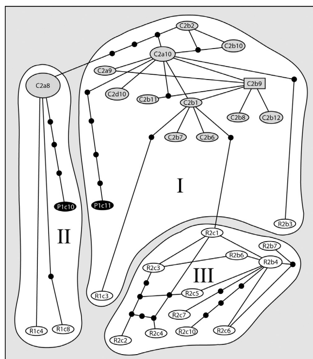
Fig. 1. Unrooted parsimony network of 30 ITS rDNA haplotypes of Diploastrea heliopora , representing a 95% plausible set of cladograms. The square represents the haplotype with the highest outgroup probability and the size of the square and ovals correspond with the haplotype frequency. On the connecting lines, each filled circle represents one step linking two haplotypes. To some extent, the ITS rDNA haplotypes are segregated according to their natal sites and have thus been arranged to reflect this geography, i.e. with the haplotypes to the top of the figure originating from Cyrene Reef (C prefix, light shading) and the haplotypes to the bottom of the figure coming from Raffles Lighthouse (R prefix, no shading). The two haplotypes from Pulau Hantu (P prefix, dark shading) have been placed in the middle. Three haplotype clades (I, II and III) are outlined.
