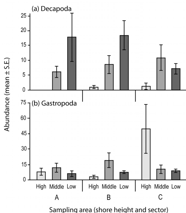
Fig. 4. Bar charts showing mean abundance of decapods (a), and gastropods (b), at each sampling area. Error bars denote standard errors.
