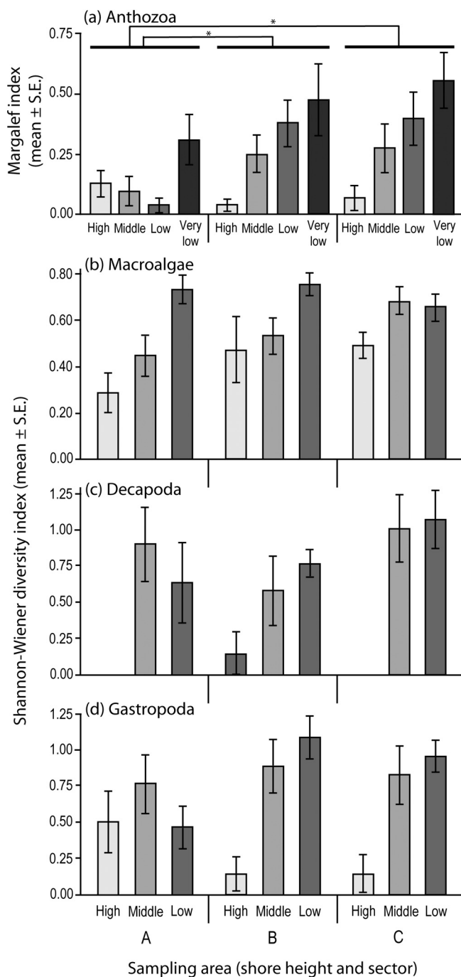
Fig. 2. Bar charts showing mean Margalef index scores of anthozoans (a), and Shannon-Wiener index scores of macroalgae (b), decapods (c), and gastropods (d), at each sampling area. Error bars denote standard errors. Differences between sectors, as revealed by Student-Newman-Keuls tests, are indicated above each graph.
