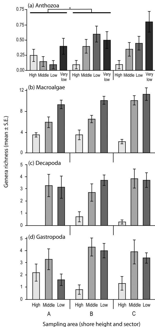
Fig. 3. Bar charts showing mean genera richness of anthozoans (a), macroalgae (b), decapods (c), and gastropods (d), at each sampling area. Error bars denote standard errors. Differences between sectors, as revealed by Student-Newman-Keuls tests, are indicated above each graph.
