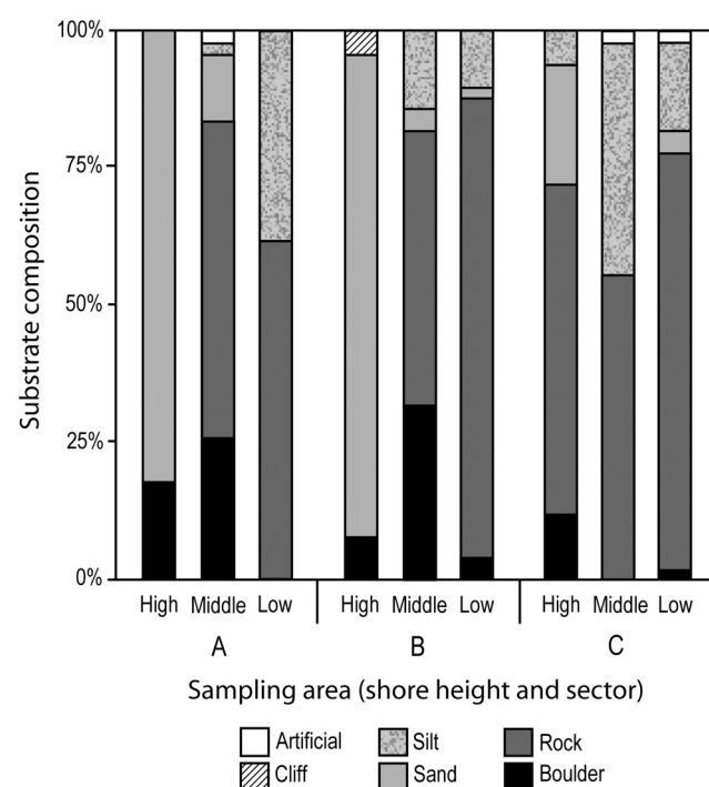
Fig. 5. Substrate composition at each of nine sampling areas.
